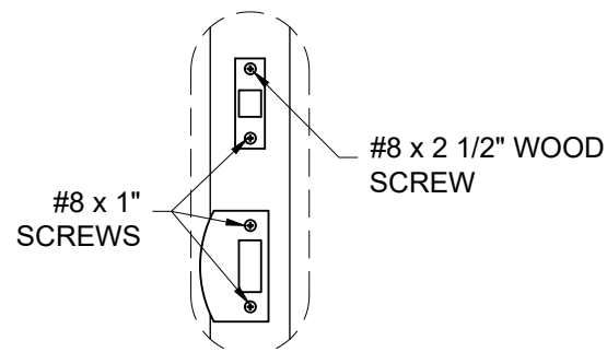
ENTRY DOOR STRIKE DETAIL WOOD FRAME SUBSTRATE
