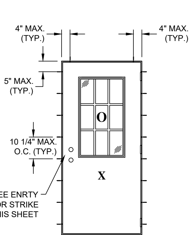
ENTRANCE DOOR ANCHOR LAYOUT
